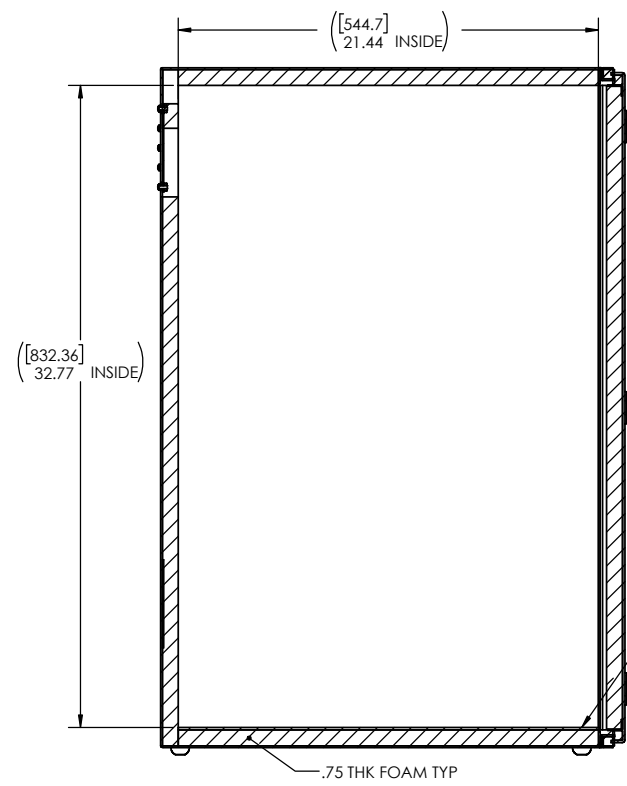
SECTION C-C SCALE 1 : 4.9
